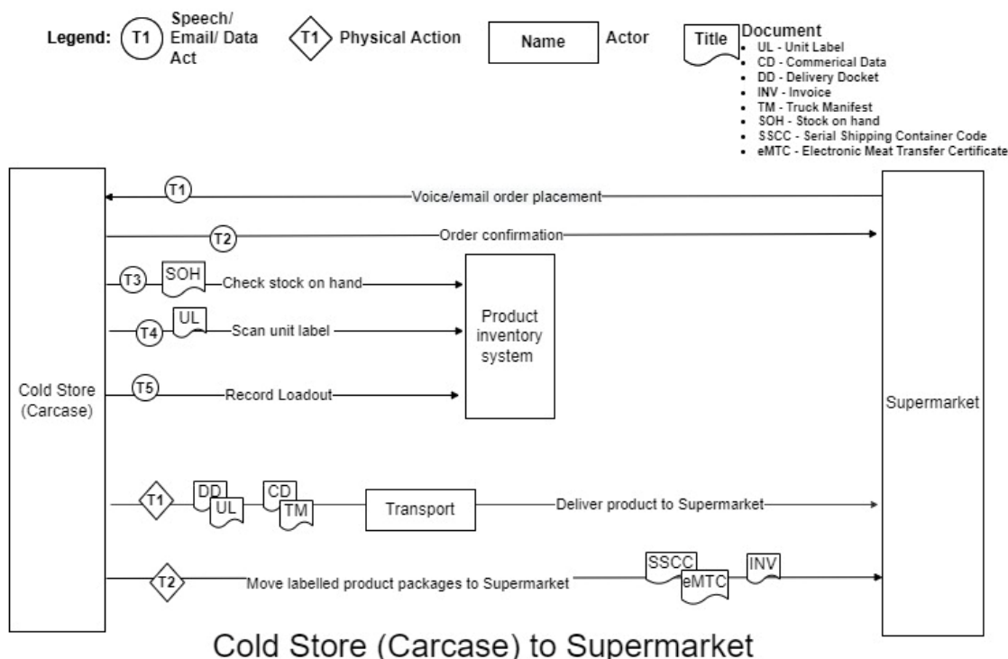
Figure 119 Data or information flows from the cold store (carcase) supermarket systems in the beef supply chain.
