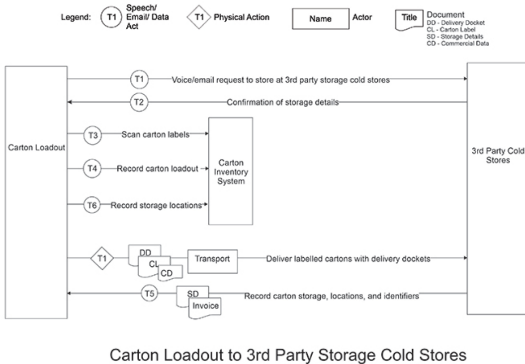
Figure 181. Data or information flows from the import carton loadout to import third party cold store systems in the beef supply chain.
