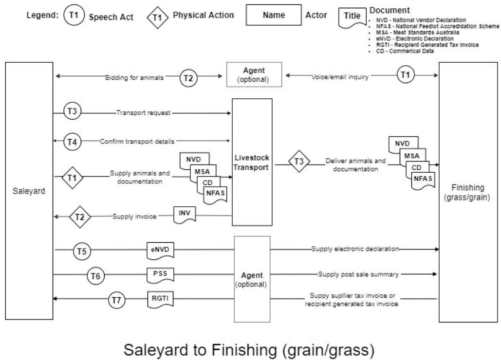
Figure 22. Data or information flows from the saleyard to finishing (grain or grass) systems in the beef supply chain.
