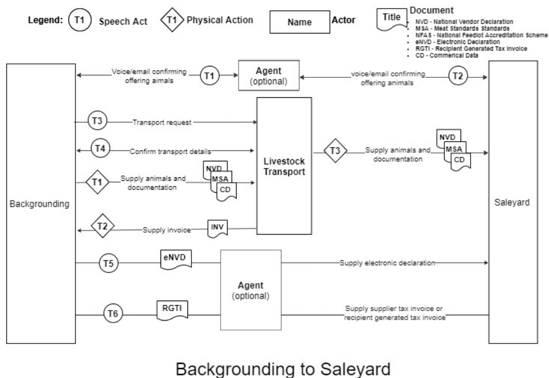
Figure 27. Data or information flows from the backgrounding to saleyard systems in the beef supply chain.
