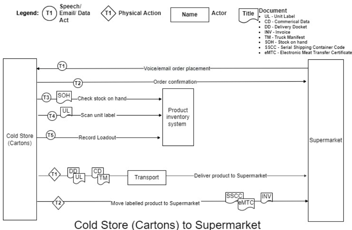
Figure 120 Data or information flows from the cold store (carton) to supermarket systems in the beef supply chain.
