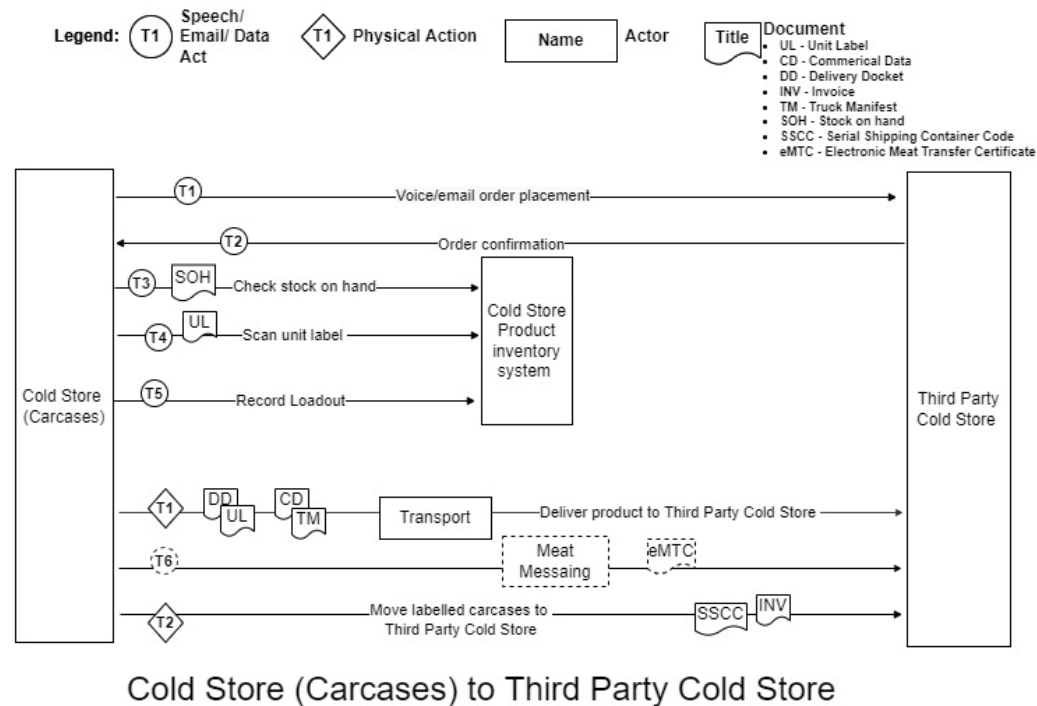
Figure 112 Data or information flows from the cold store (carcasses) loadout to third-party cold store systems in the beef supply chain.
