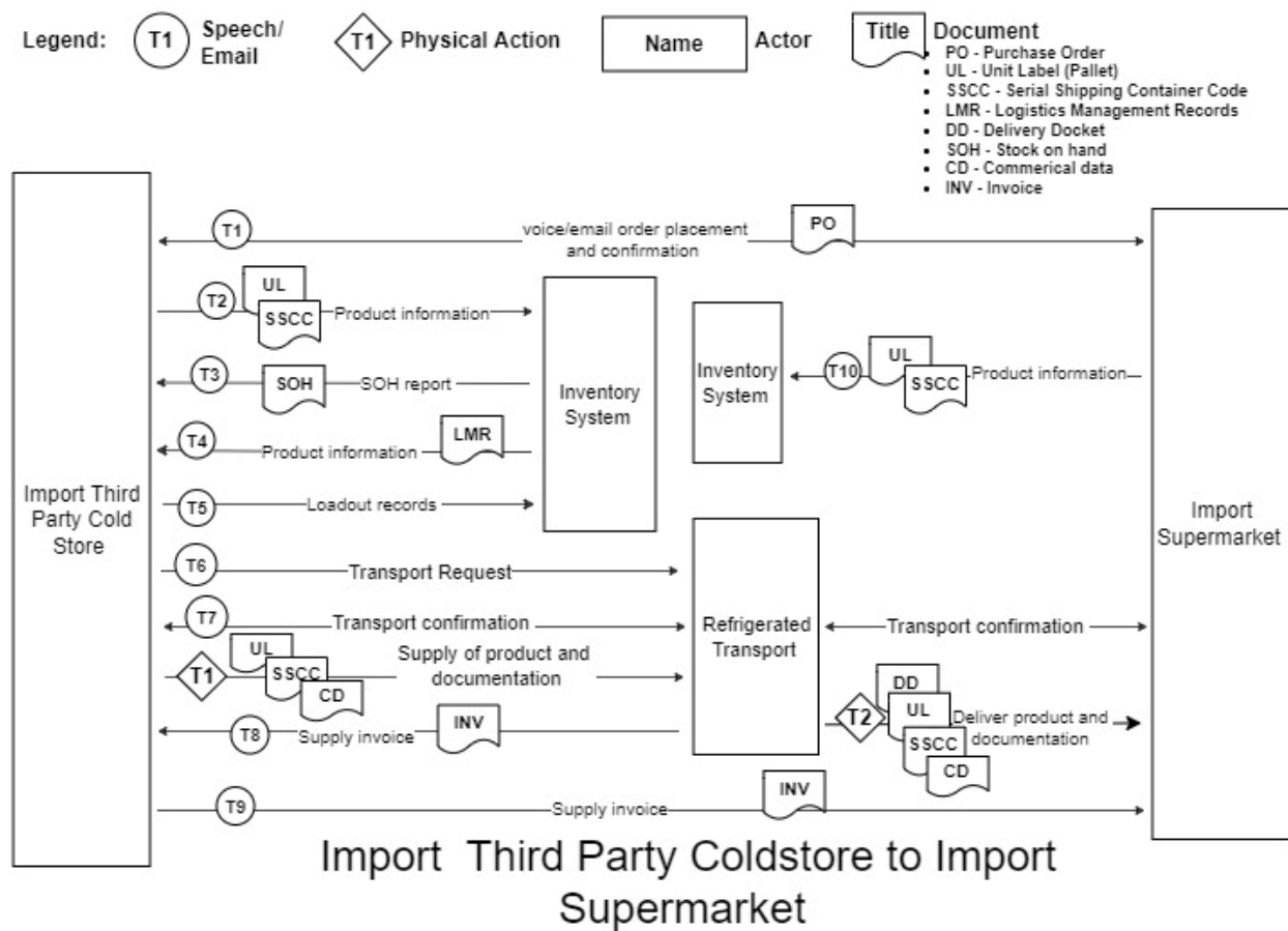
Figure 197. Data or information flows from the import third party cold store to import supermarkets systems in the beef supply chain
