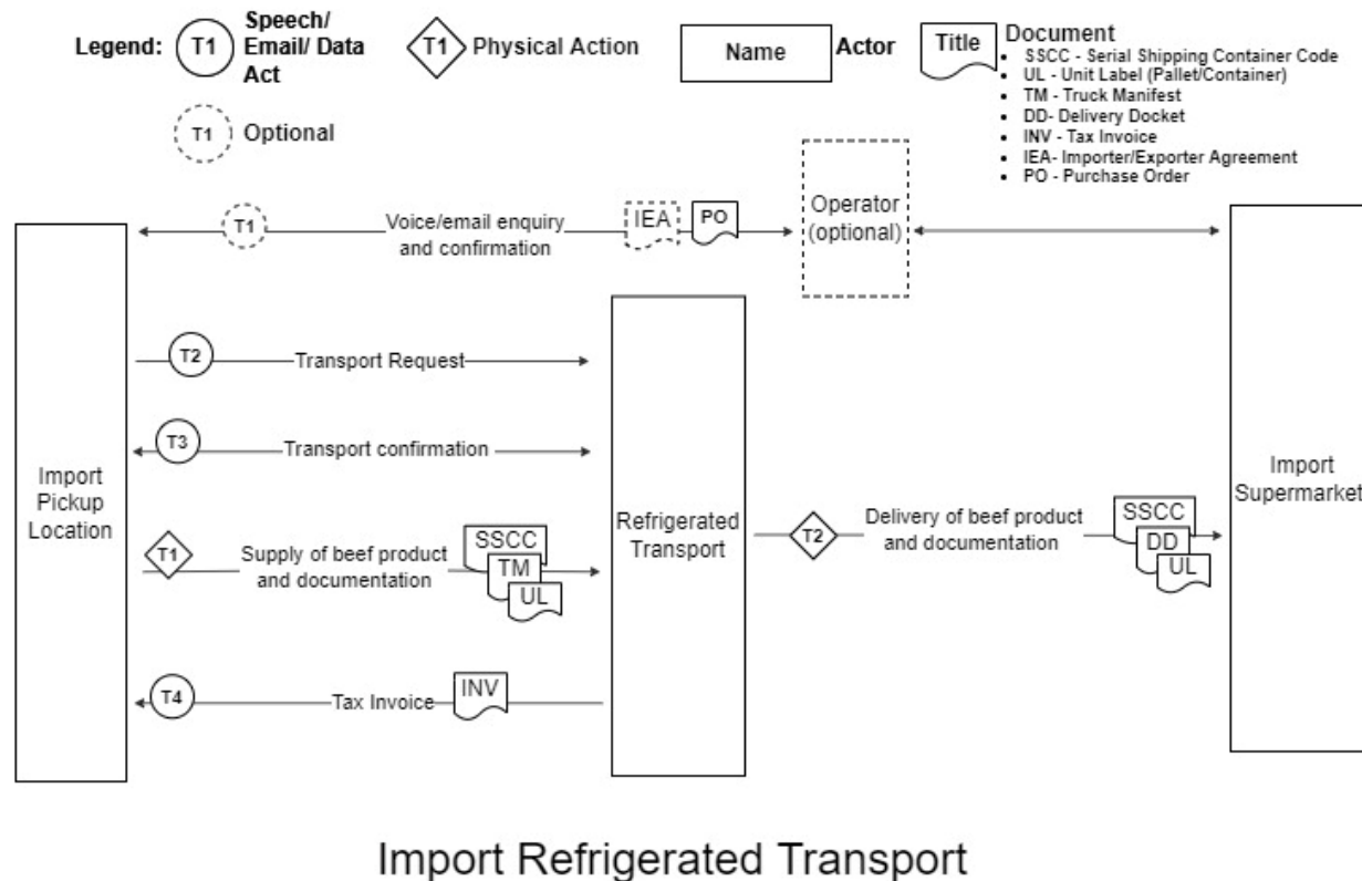
Figure 188. Data or information flows from import refrigerated transport systems in the beef supply chain.
