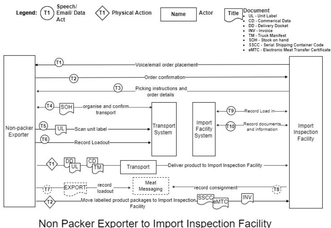
Figure 155. Data or information flows from the non-packer exporter to import inspection facility systems in the beef supply chain.
