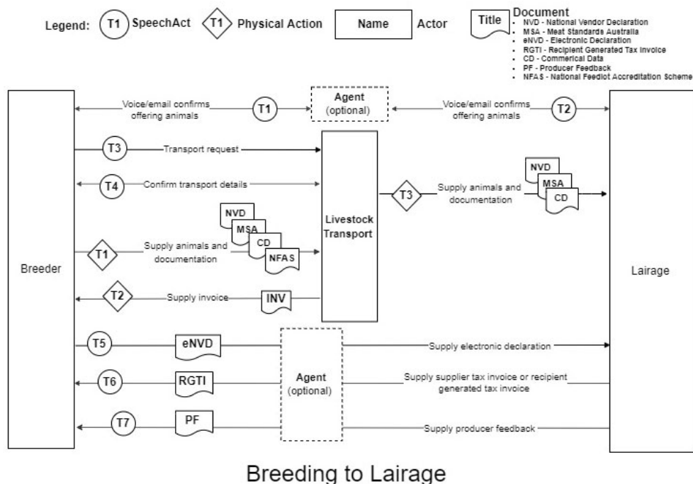
Figure 9. Data or information flows from the breeding to lairage systems in the beef supply chain.
