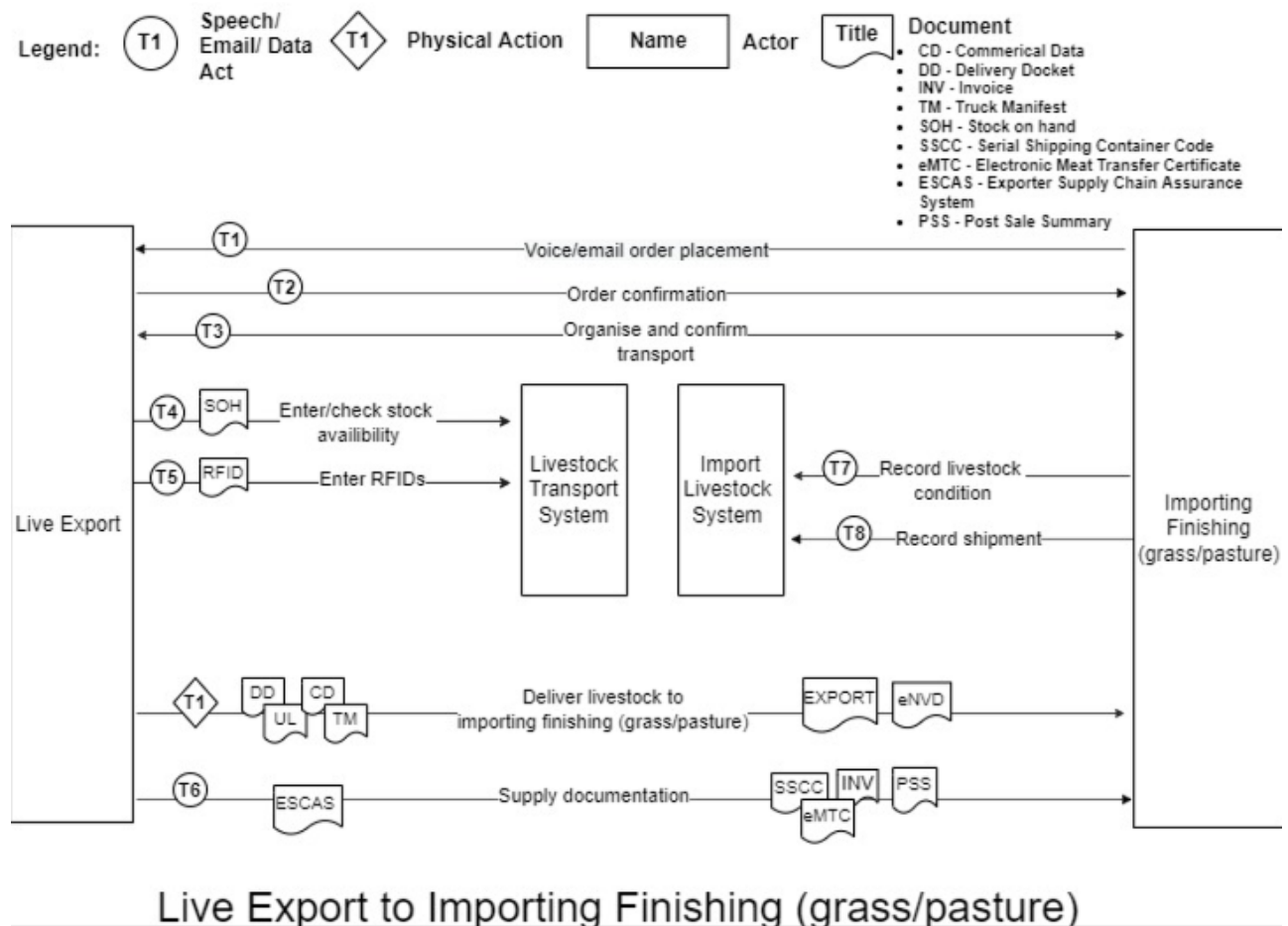
Figure 165. Data or information flows from live export to import finishing (grass/pasture) systems in the beef supply chain
