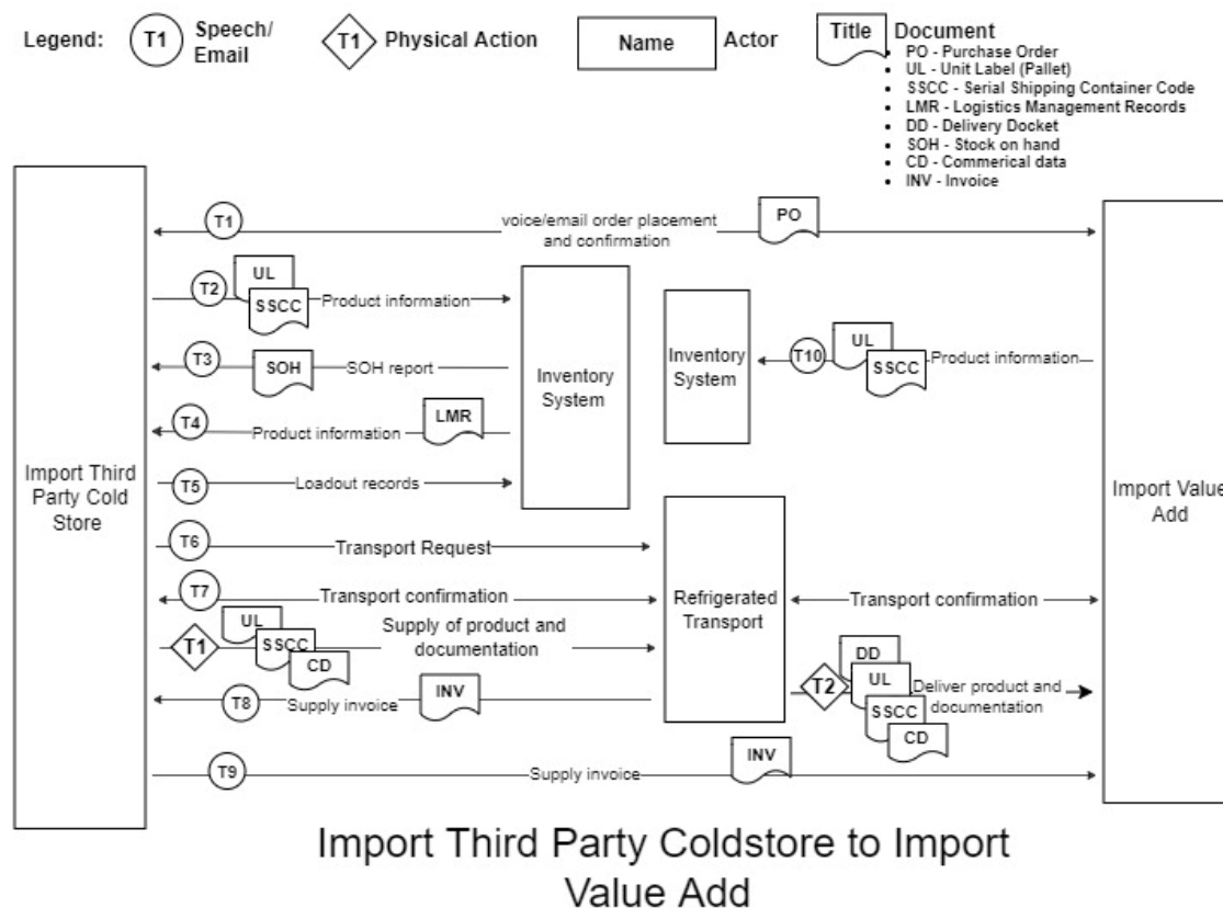
Figure 175. Data or information flows from import third party cold store to import value add systems in the beef supply chain.
