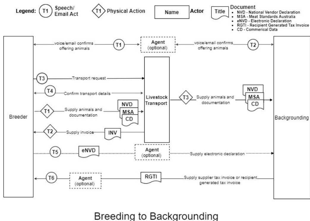
Figure 8. Data or information flows from the breeding to backgrounding systems in the beef supply chain.
